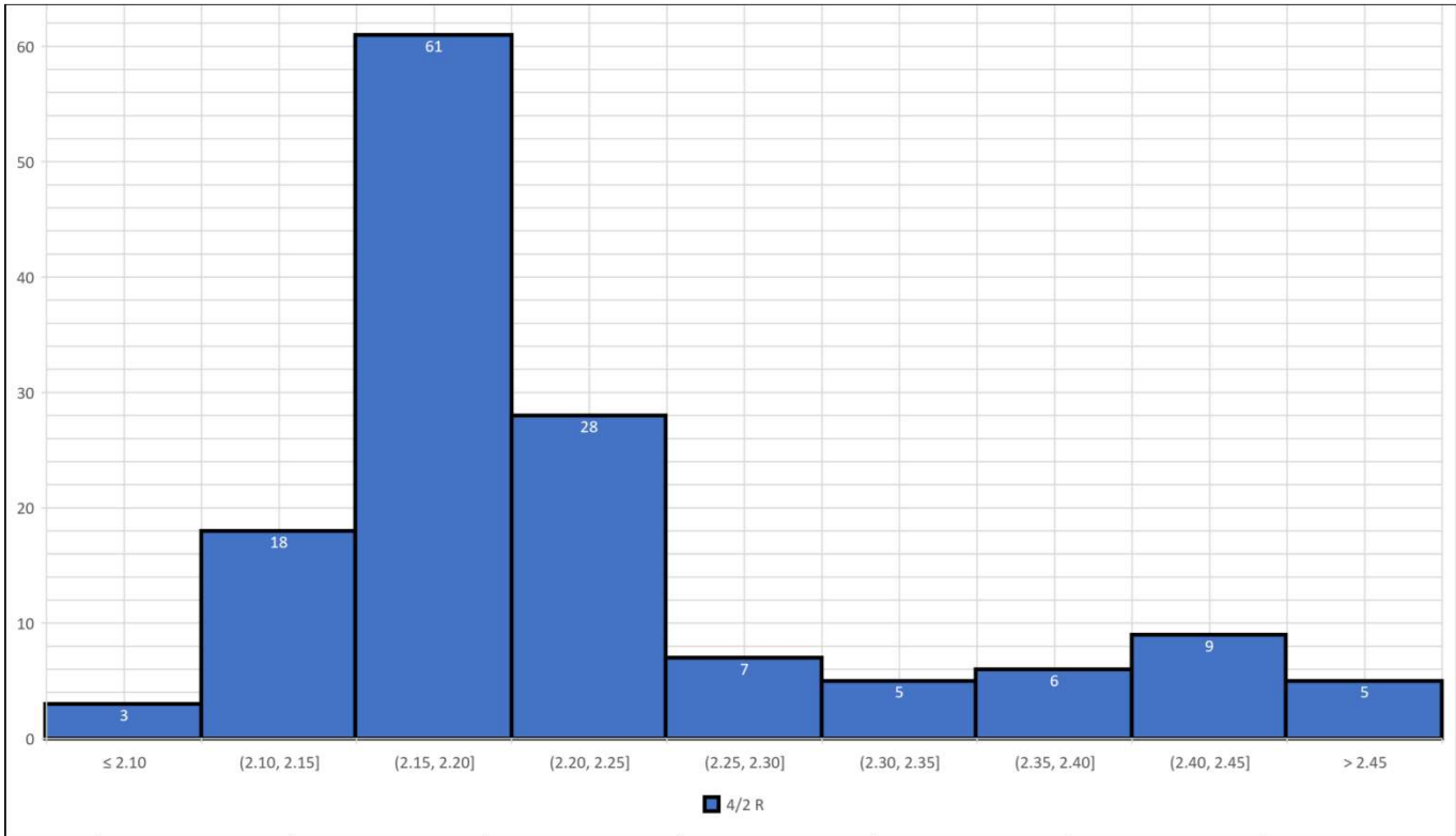
ERROR HISTOGRAM
