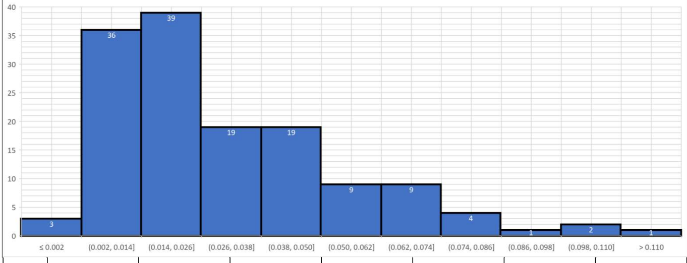
ERROR HISTOGRAM
